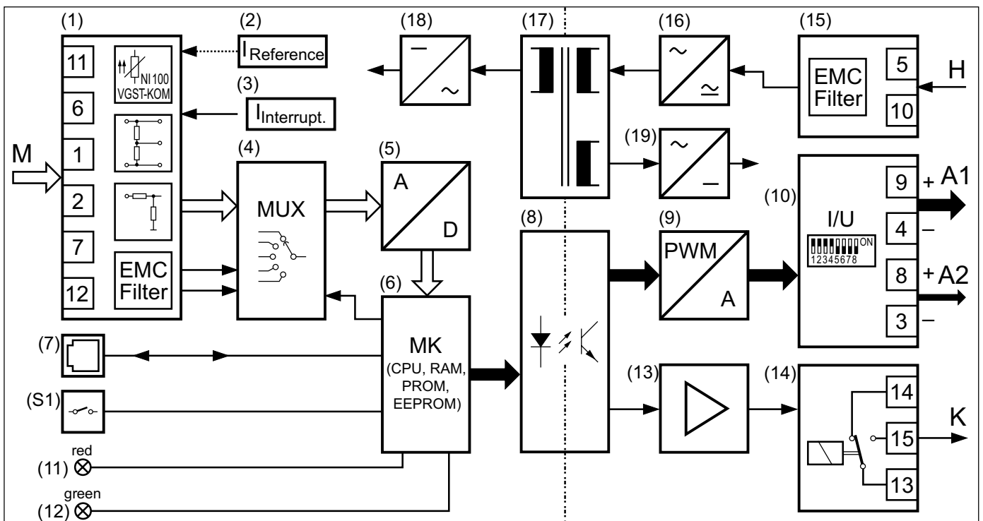
Fig. 3. Block diagram. I
