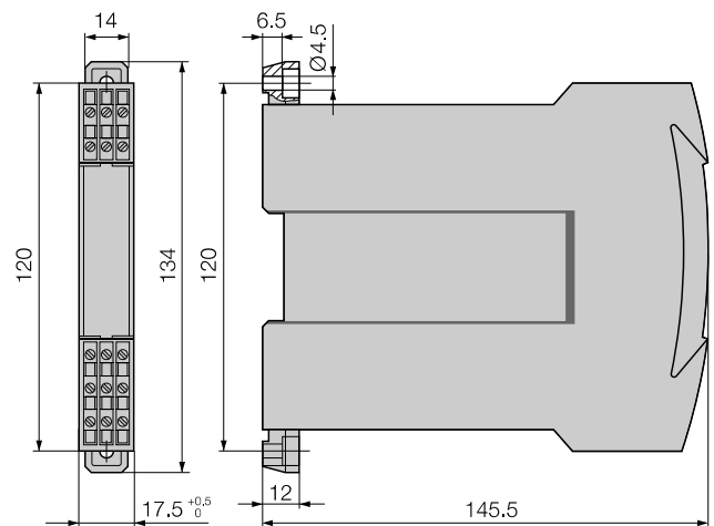
Fig 11. ZIEGLER TV 808 in housing S17, screw hole mounting brackets pulled out.
