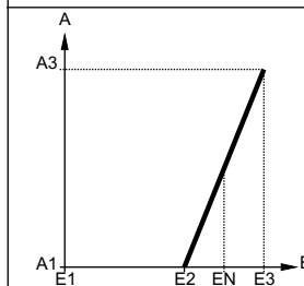
Fig. 7. Characteristic B "Current resp. voltage magnifier in end range". E1...E2 suppressed completely, E2...E3 (main measuring range) magnified Condition: \frac{E3}{E2} = 1.22...1.66
