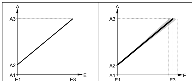
Fig. 5. Characteristic A "Standard and live zero". Condition: A2 = 0.2 A3
