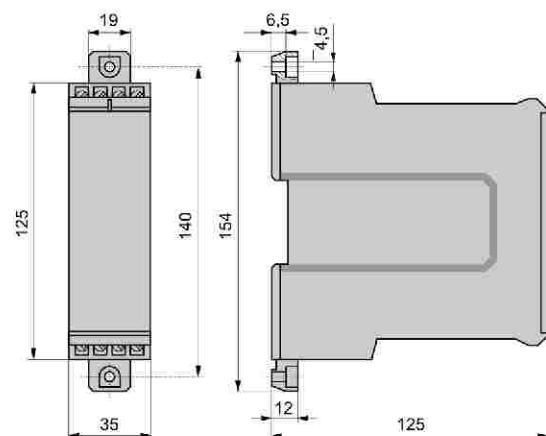
Fig. 13. Transducer with the screw hole brackets pulled out for wall mounting.
