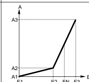
Fig. 8. Characteristic C "Main value magnification in end range". E1...E2 (secondary measuring range) suppressed, E2...E3 (main measuring range) magnified Conditions: \frac{E3}{E2} = 1.22...1.66
